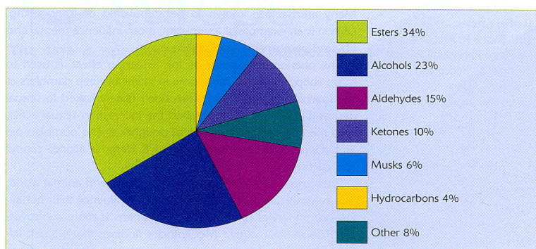
Figure 3 - Fragrances by chemical type
