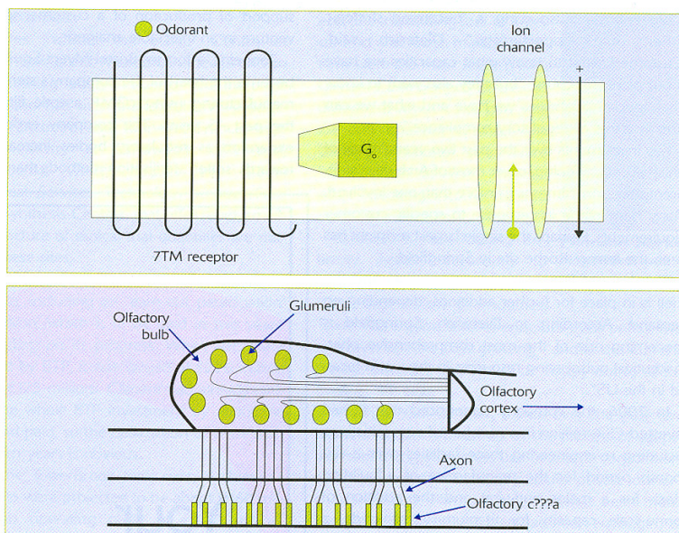
Figure 2 - Initial response to odour (top) & odour response in the brain (above)
