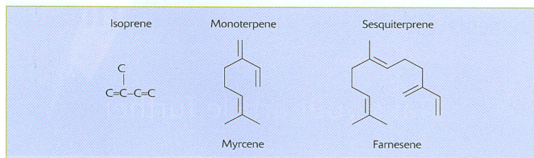
Figure 5 - (right) Macrocyclic musks
